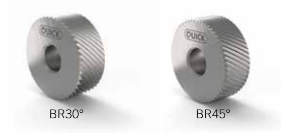
QUICK knurling wheels according to DIN 403 for profiles according to DIN 82, with 45° chamfer, PM
